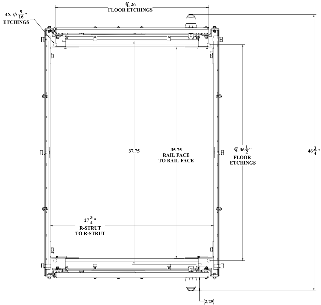
TOP VIEW NO CEILING OR ALUMASHIELD SHOWN
